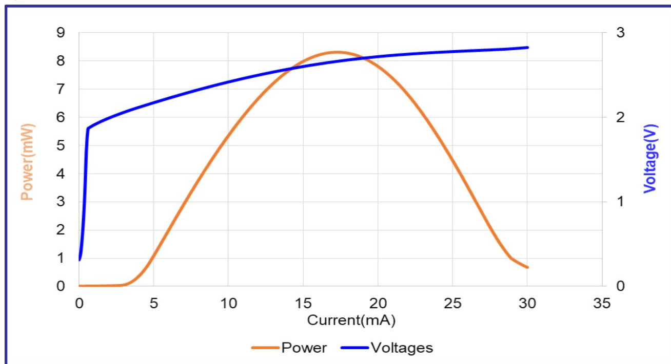
Typical Performance Curves at 25°C
